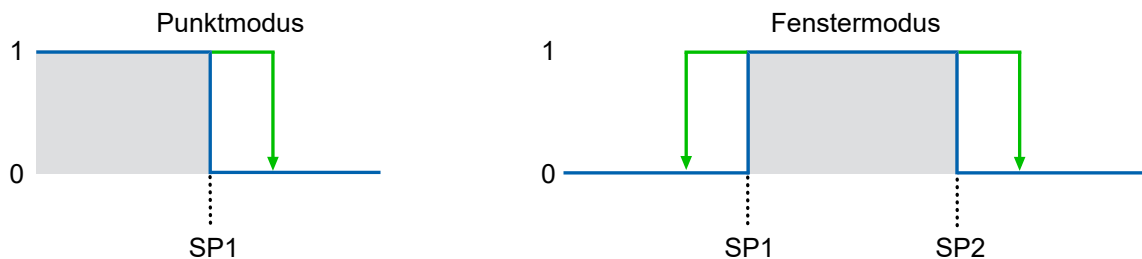
Abb. 10: Positive Hysterese
