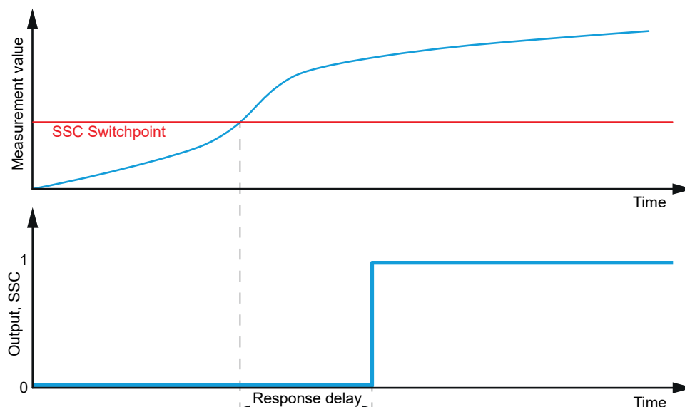
Fig. 2: Response Delay
