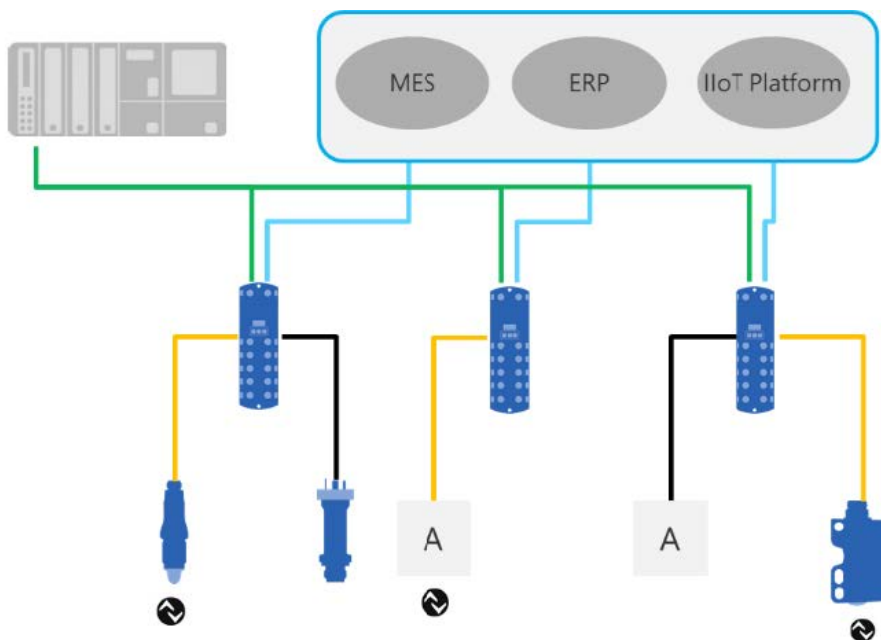
Fig. 1: Architecture IO-Link
